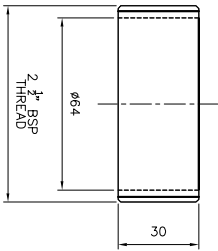
(SCALE:1:4) DETAIL-A BUSH FOR COUPLER
